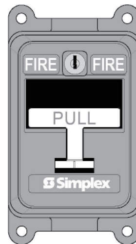
Figure 3: 2099-9144 Explosion-Proof and Weather-Proof Manual Station
